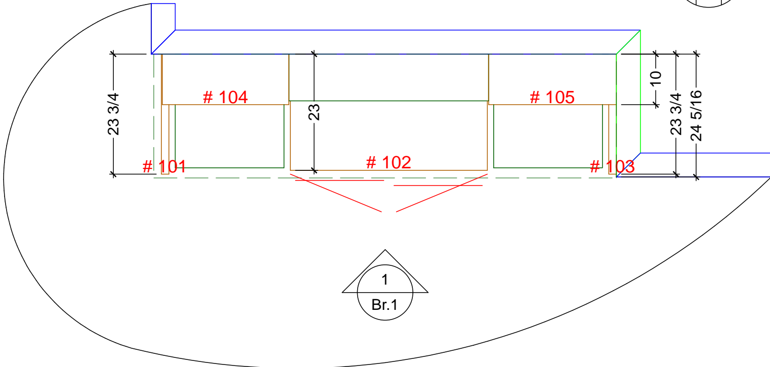
1 BAR CABINETRY FLOOR PLAN SCALE: 5/8" = 1' 0"
