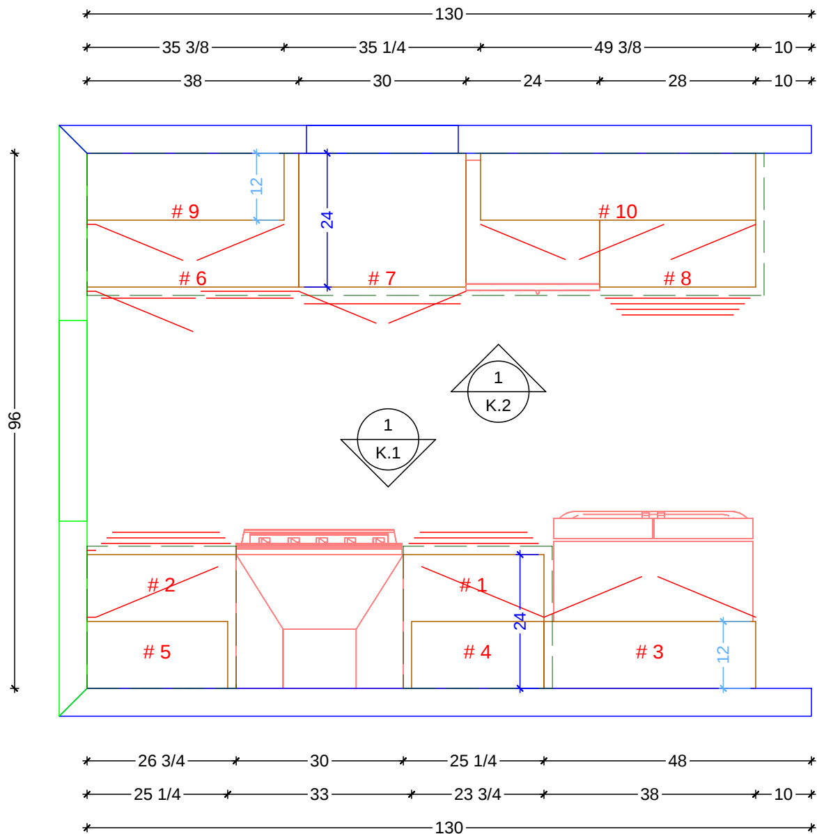
PROPOSED CABINETRY FLOOR PLAN SCALE: 1/2" = 1' 0"
