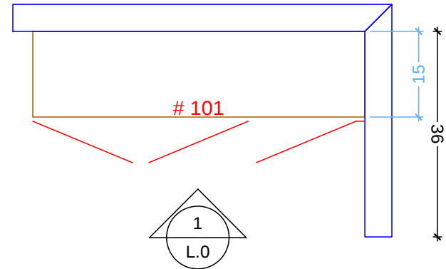
LAUNDRY CABINETRY FLOOR PLAN SCALE: 1/2" = 1' 0"
