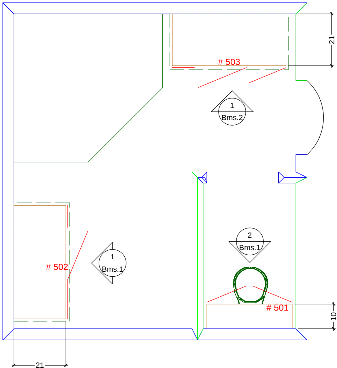
BATH-Master CABINETRY FLOOR PLAN SCALE: 1/2" = 1' 0"
