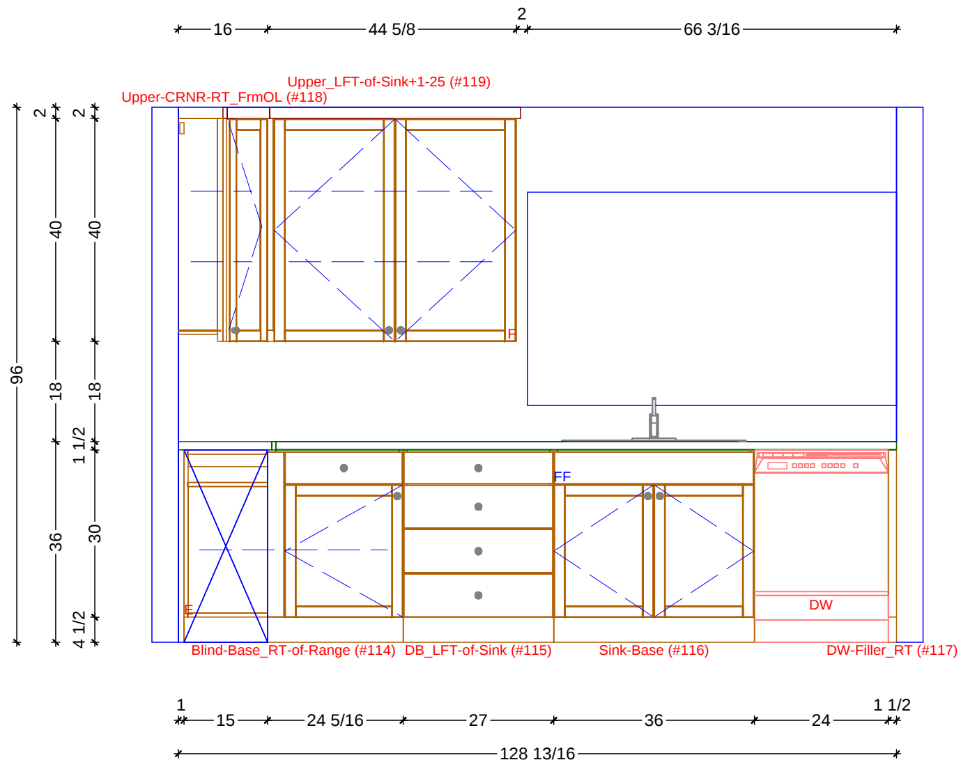
1 KITCHEN ELEVATION - WEST SCALE: 1/2" = 1' 0"
