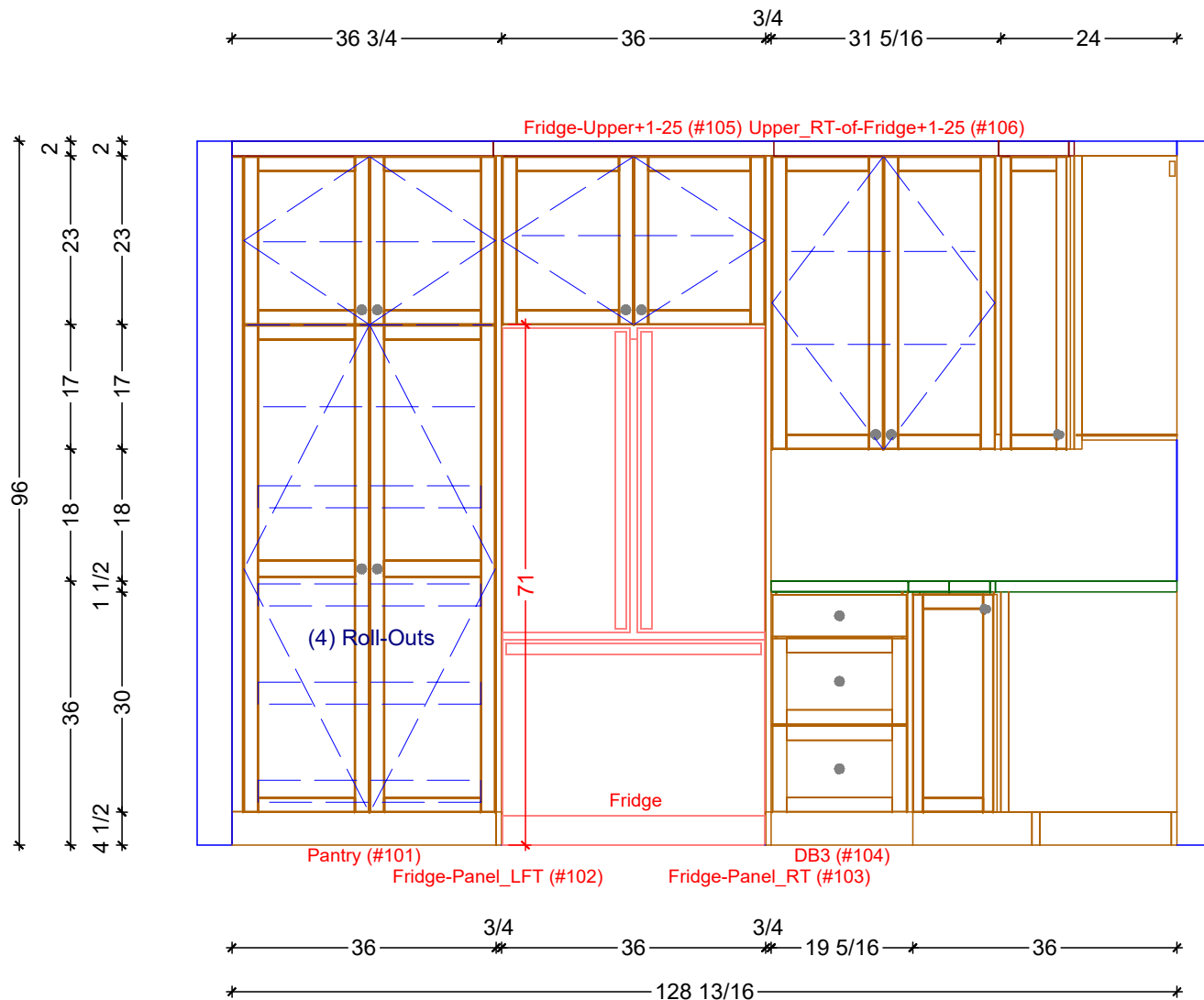
1 KITCHEN ELEVATION - EAST SCALE: 1/2" = 1' 0"
