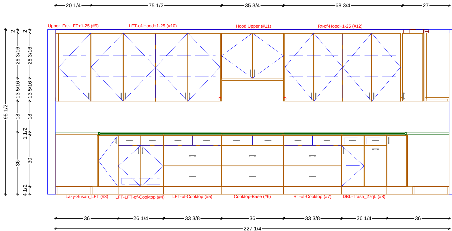
1 KITCHEN ELEVATION - COOKTOP RUN SCALE: 3/8" = 1' 0"
