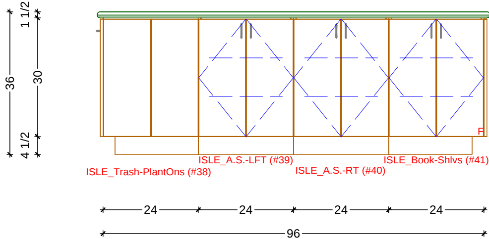
3 KITCHEN ELEVATION - ISLE - BACK SCALE: 1/2" = 1' 0"
