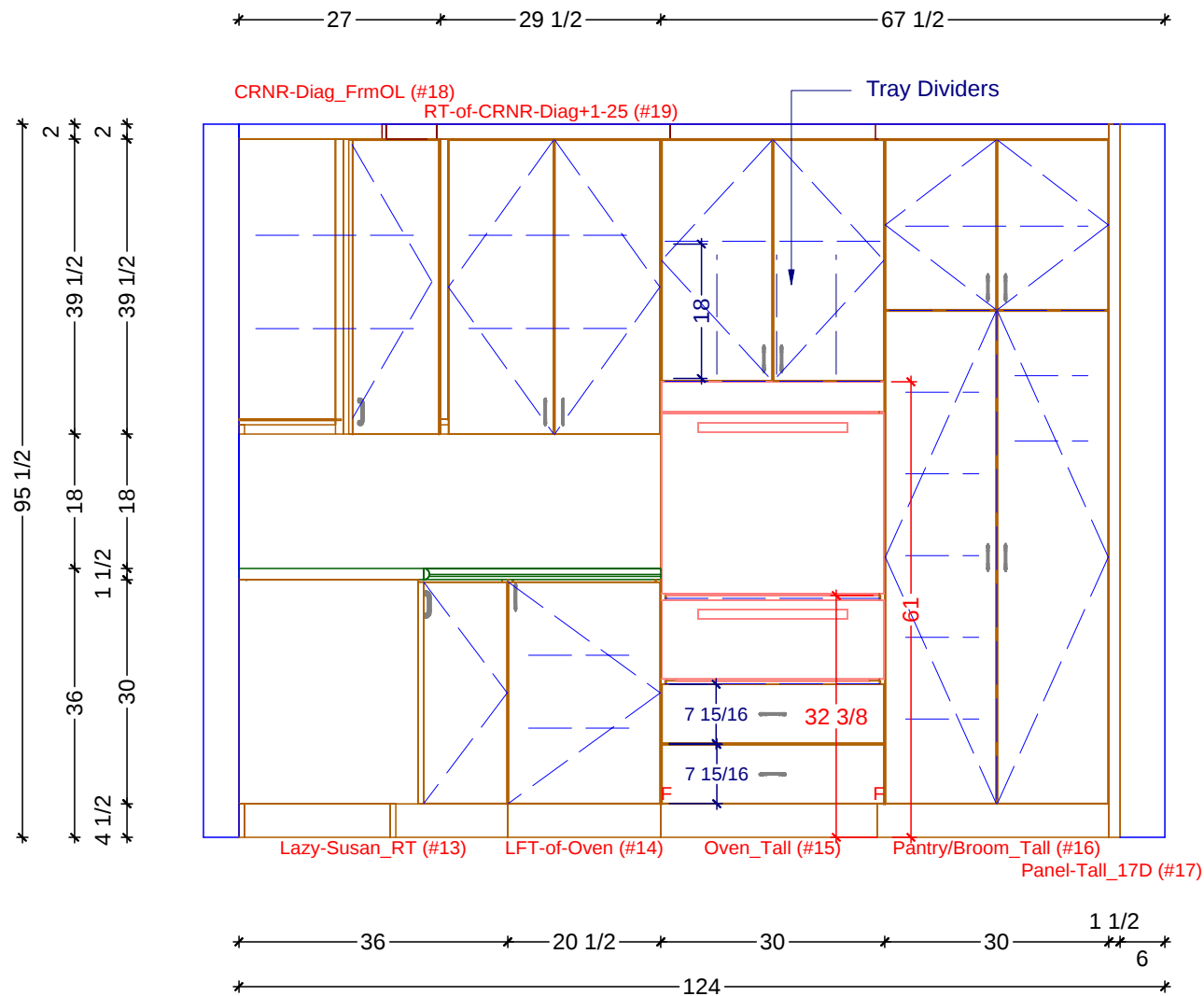
1 KITCHEN ELEVATION - OVEN RUN SCALE: 1/2" = 1' 0"
