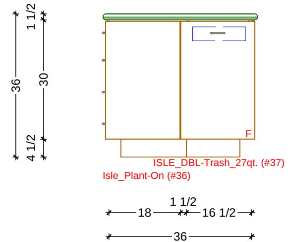
2 KITCHEN ELEVATION - ISLE - END SCALE: 1/2" = 1' 0"
