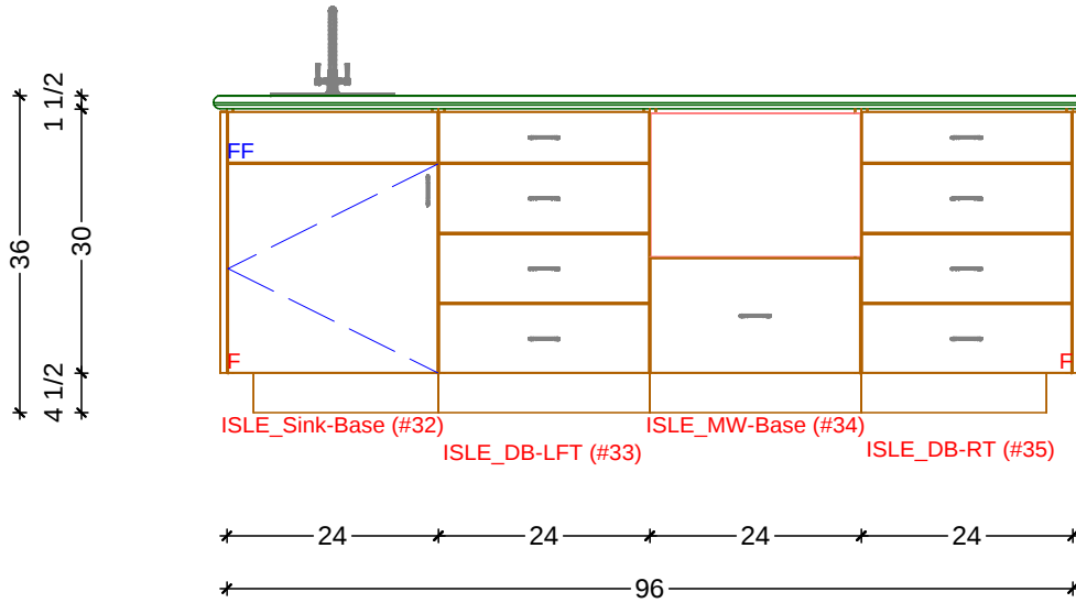
1 KITCHEN ELEVATION - ISLE - FRONT SCALE: 1/2" = 1' 0"
