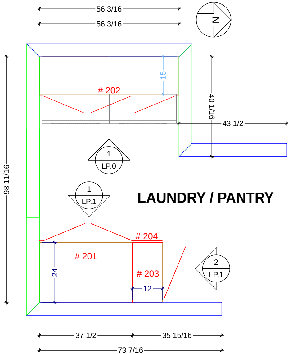
LAUNDRY-PANTRY CABINETRY FLOOR PLAN SCALE: 1/2" = 1' 0"
