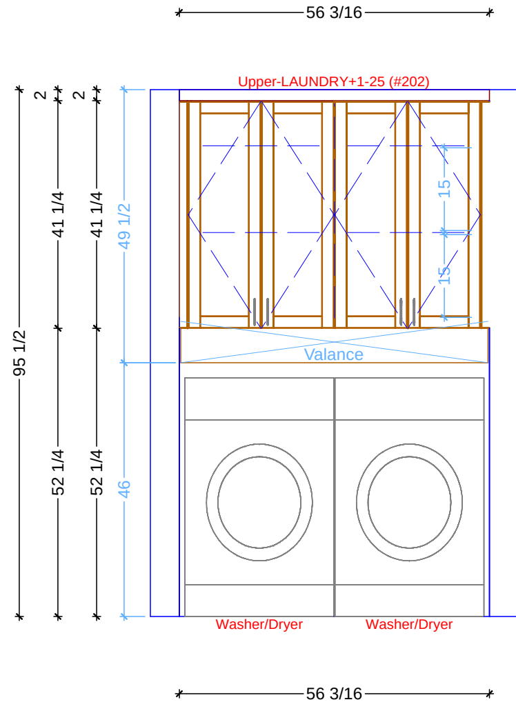
1 LAUNDRY-PANTRY ELEVATION - WEST SCALE: 1/2" = 1' 0"
