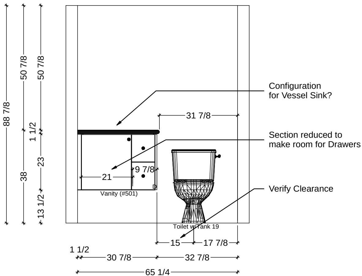
1 BATH-HALLWAY ELEVATION - NORTH SCALE: 1/2" = 1' 0"
