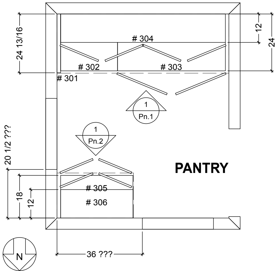
PANTRY CABINETRY FLOOR PLAN SCALE: 1/2" = 1' 0"
