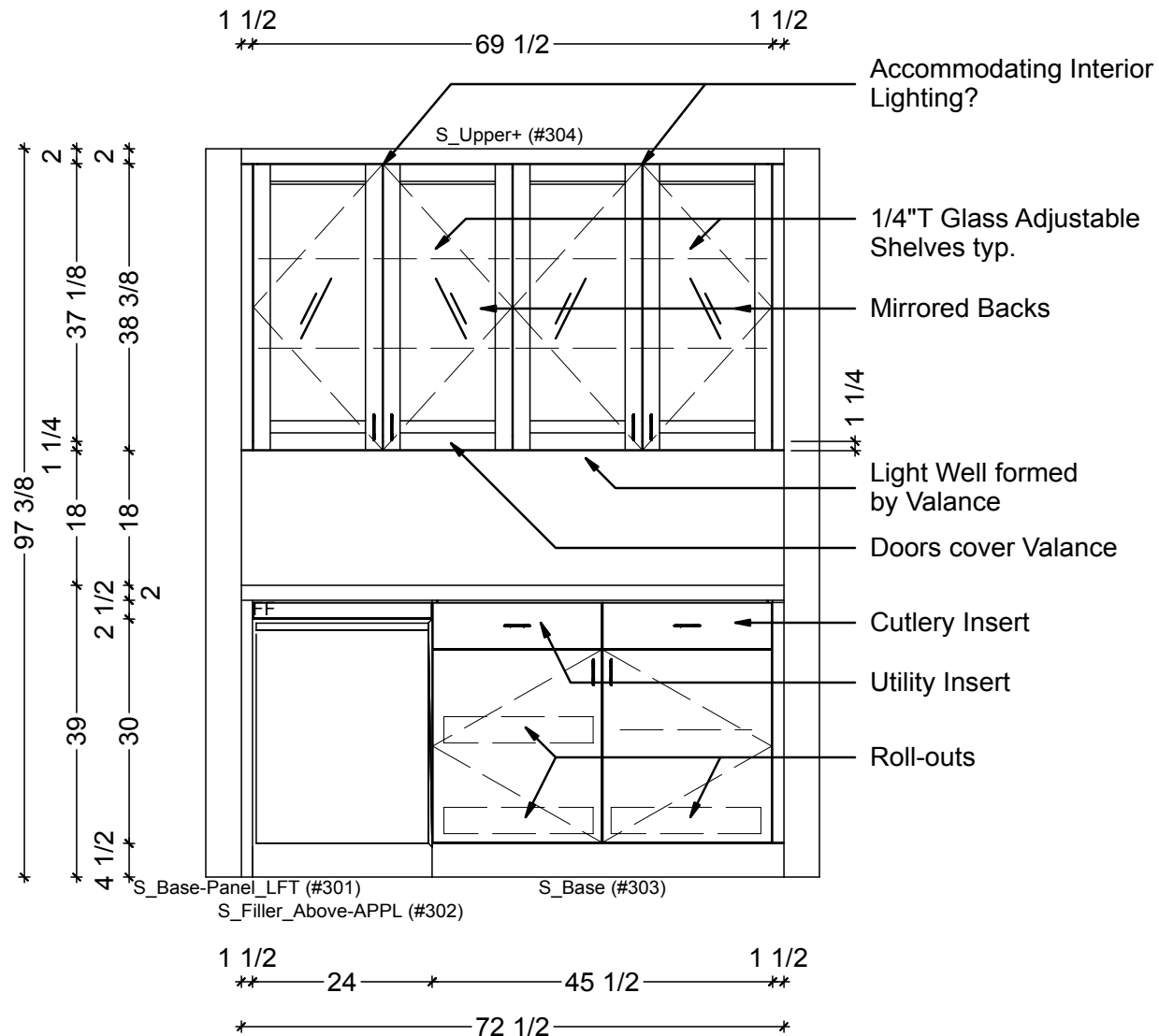
1 PANTRY ELEVATION - SOUTH SCALE: 1/2" = 1' 0"
