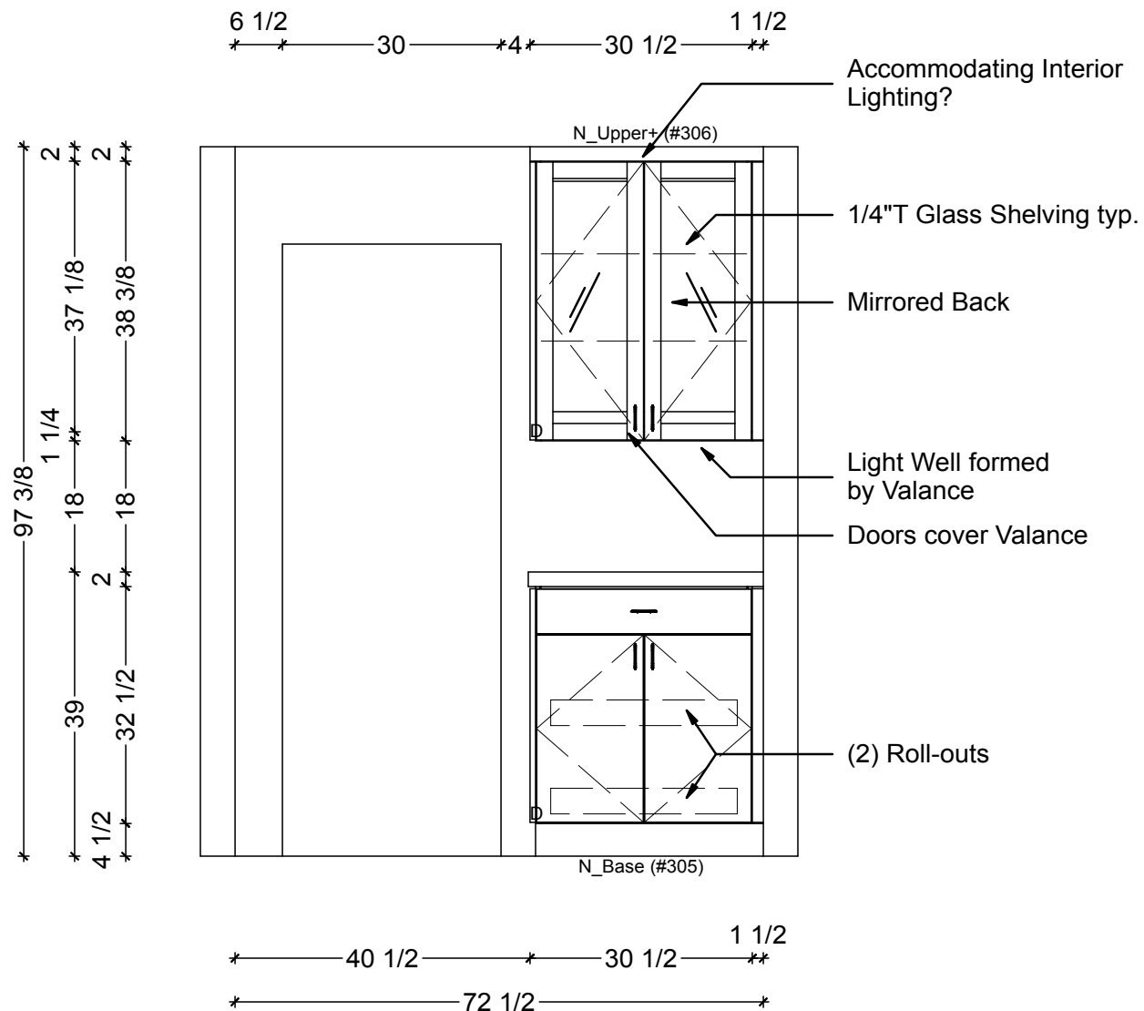
1 PANTRY ELEVATION - NORTH SCALE: 1/2" = 1' 0"
