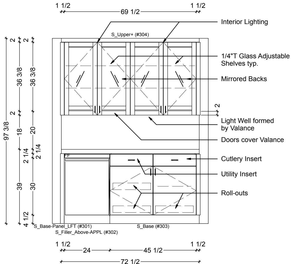
1 PANTRY ELEVATION - SOUTH SCALE: 1/2" = 1' 0"
