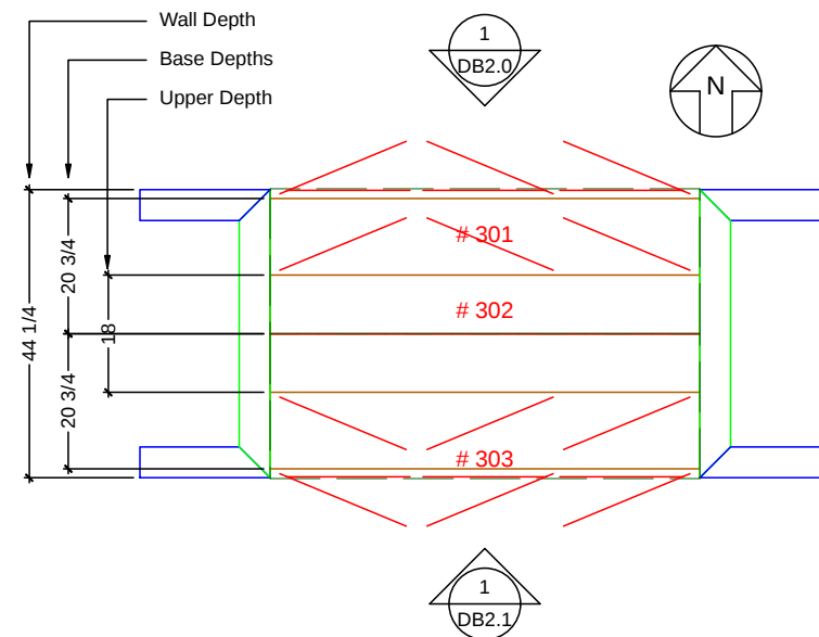
DINING-BREAKFAST2 CABINETRY FLOOR PLAN SCALE: 3/8" = 1' 0"
