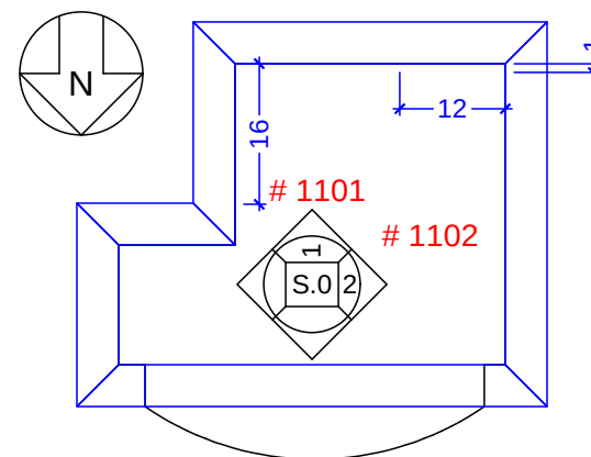
STORAGE CABINETRY FLOOR PLAN SCALE: 1/2" = 1' 0"
