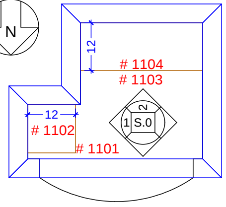
STORAGE CABINETRY FLOOR PLAN SCALE: 1/2" = 1' 0"
