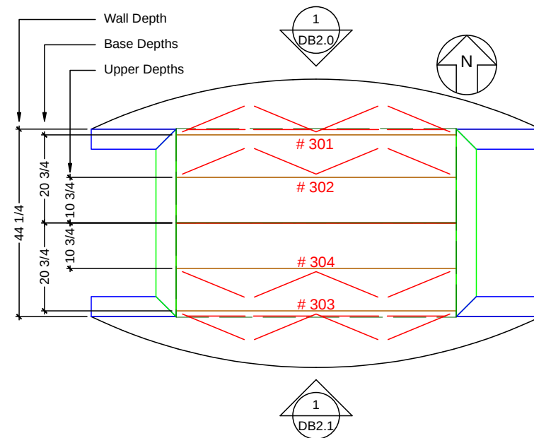
DINING-BREAKFAST2 CABINETRY FLOOR PLAN SCALE: 3/8" = 1' 0"
