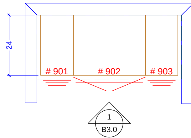
BATHROOM-3 CABINETRY FLOOR PLAN SCALE: 1/2" = 1' 0"
