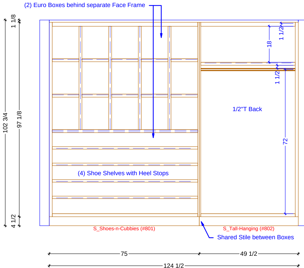
1 CLOSET-MASTER1 ELEVATION - SOUTH SCALE: 1/2" = 1' 0"
