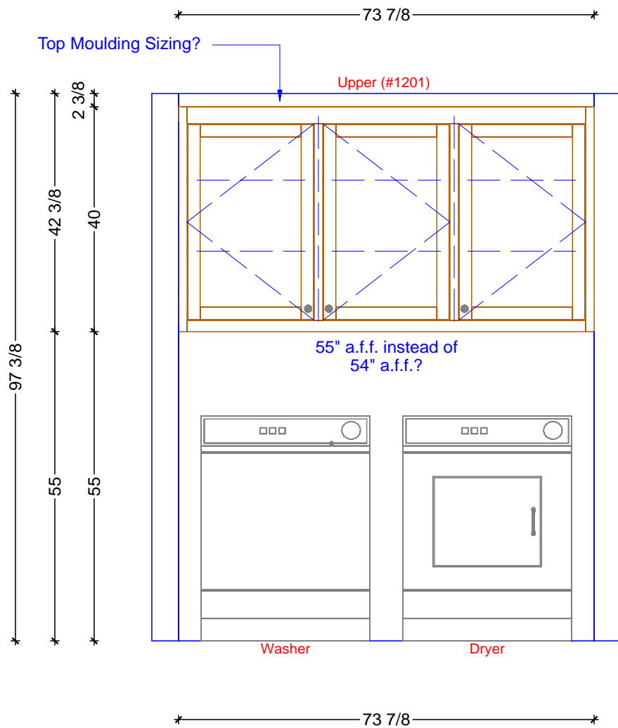
1 LAUNDRY ELEVATION - EAST SCALE: 1/2" = 1' 0"
