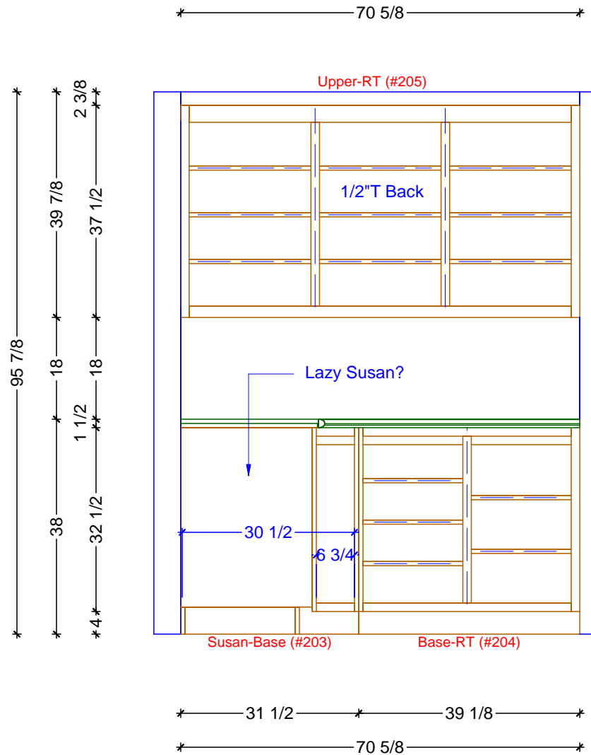
2 PANTRY ELEVATION - NORTH SCALE: 1/2" = 1' 0"
