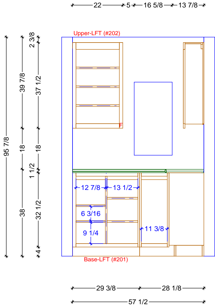
1 PANTRY ELEVATION - WEST SCALE: 1/2" = 1' 0"
