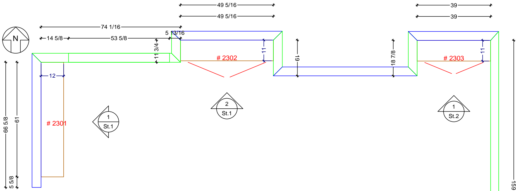
STUDY CABINETY FLOOR PLAN SCALE: 3/8" = 1' 0"
