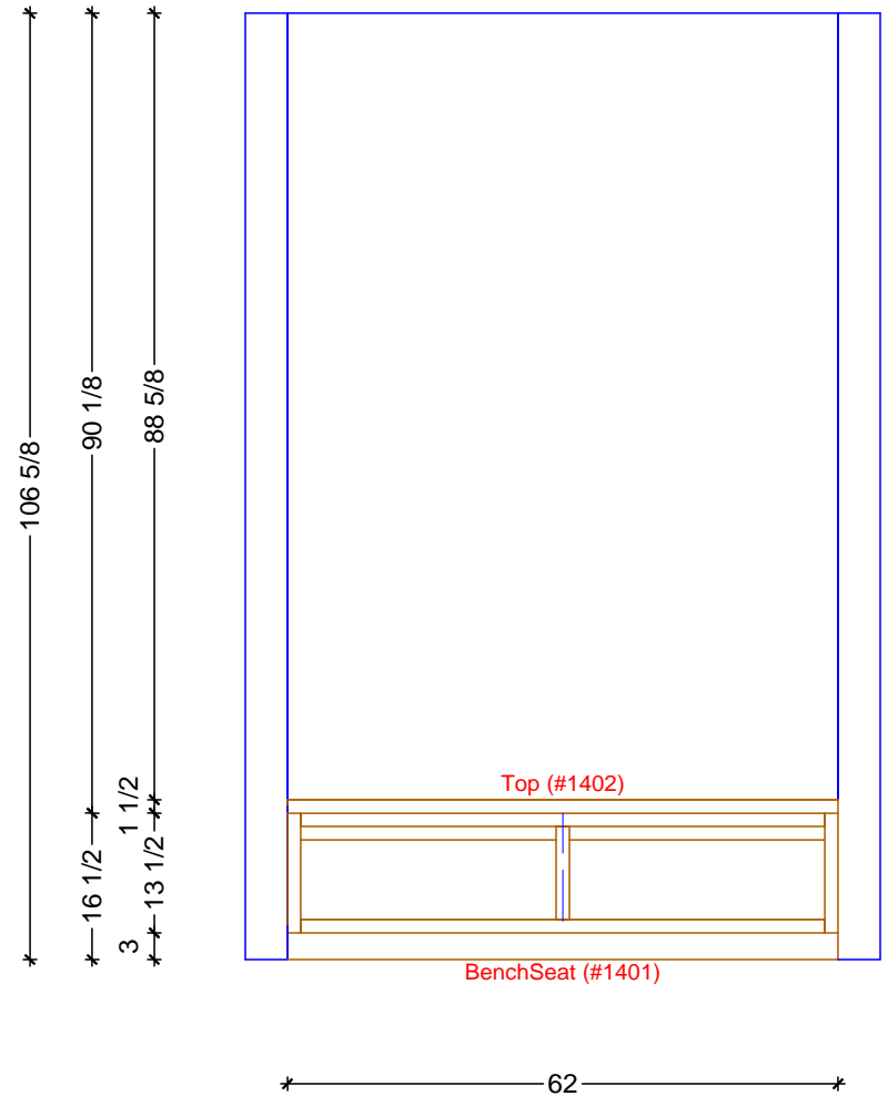
1 MUDROOM ELEVATION - EAST SCALE: 1/2" = 1' 0"
