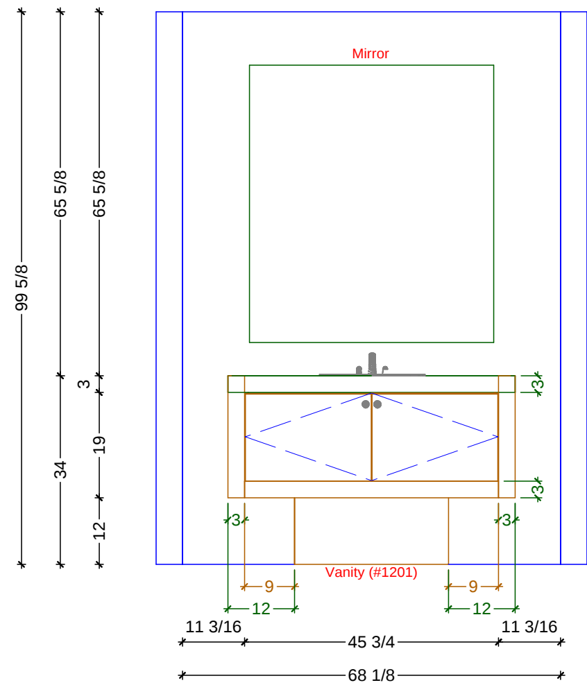
1 POWDER BATH ELEVATION SCALE: 1/2" = 1' 0"
