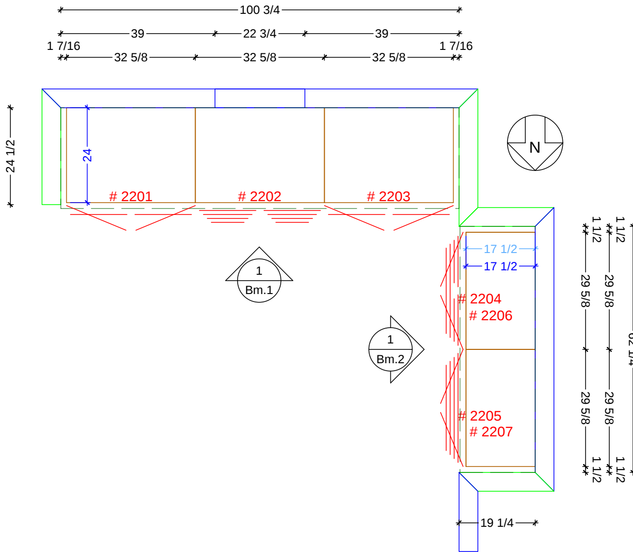
MASTER BATHROOM FLOOR PLAN SCALE: 1/2" = 1' 0"
