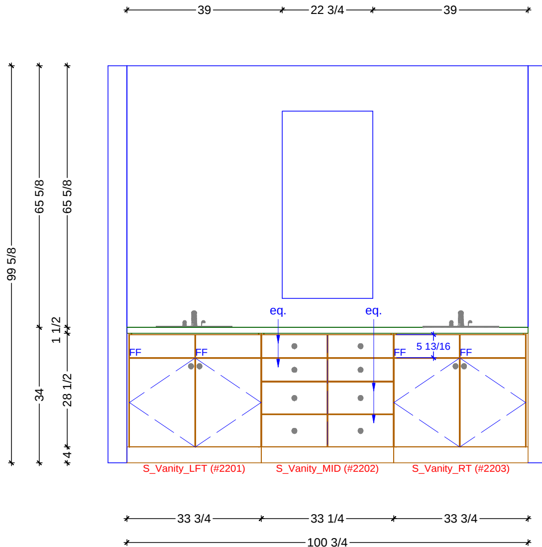
1 MASTER BATHROOM ELEVATION - SOUTH SCALE: 1/2" = 1' 0"
