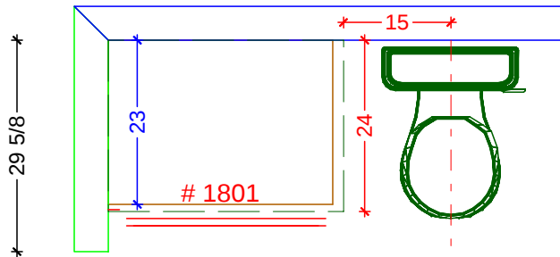
PLAN VIEW SCALE: 3/8" = 1' 0"
