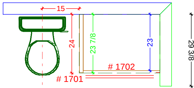
PLAN VIEW SCALE: 3/8" = 1' 0"
