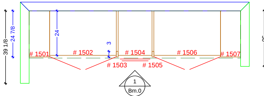
PLAN VIEW SCALE: 3/8" = 1' 0"
