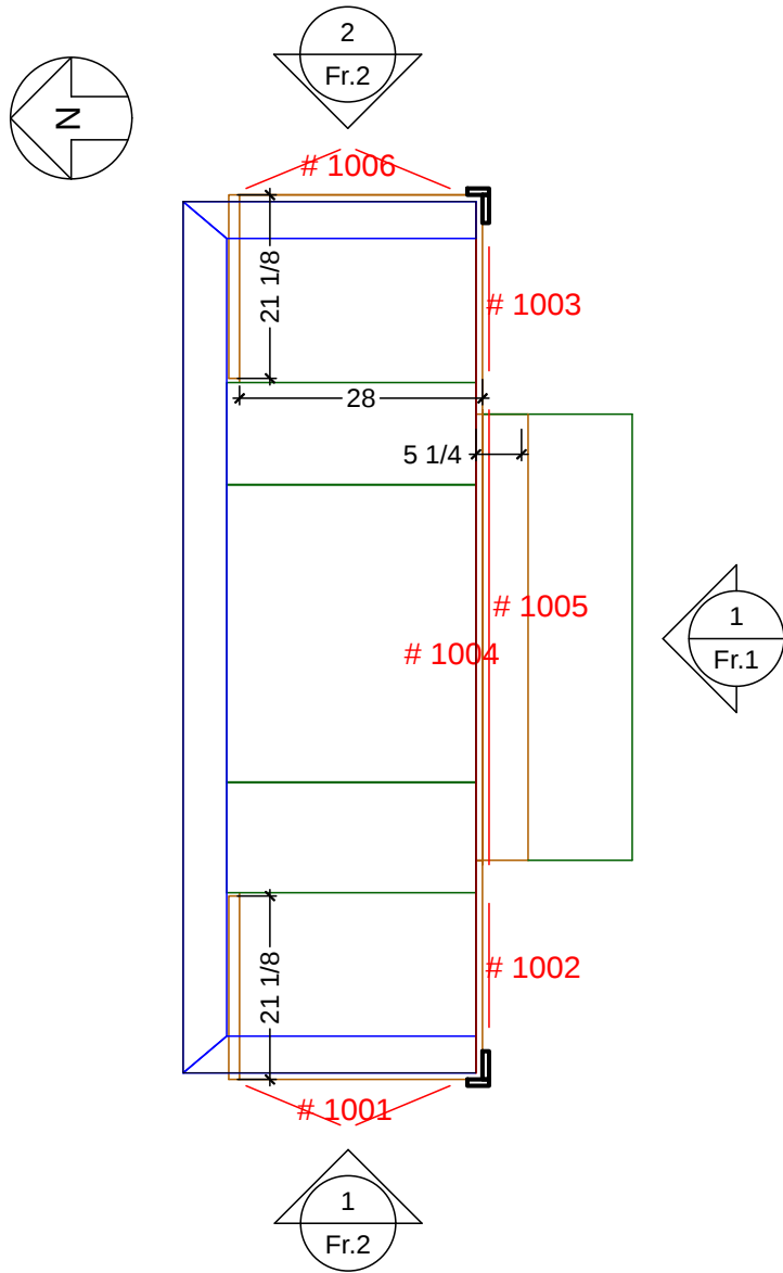
FIREPLACE CABINETRY FLOOR PLAN SCALE: 1/2" = 1' 0"
