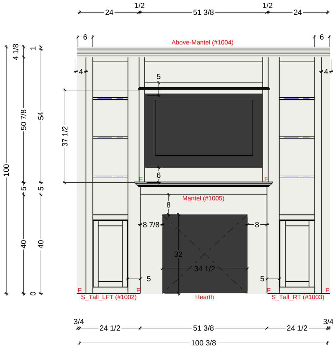
1 FIREPLACE ELEVATION - FACING NORTH SCALE: 1/2" = 1' 0"
