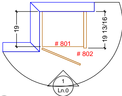
LINEN CABINETRY FLOOR PLAN SCALE: 3/8" = 1' 0"
