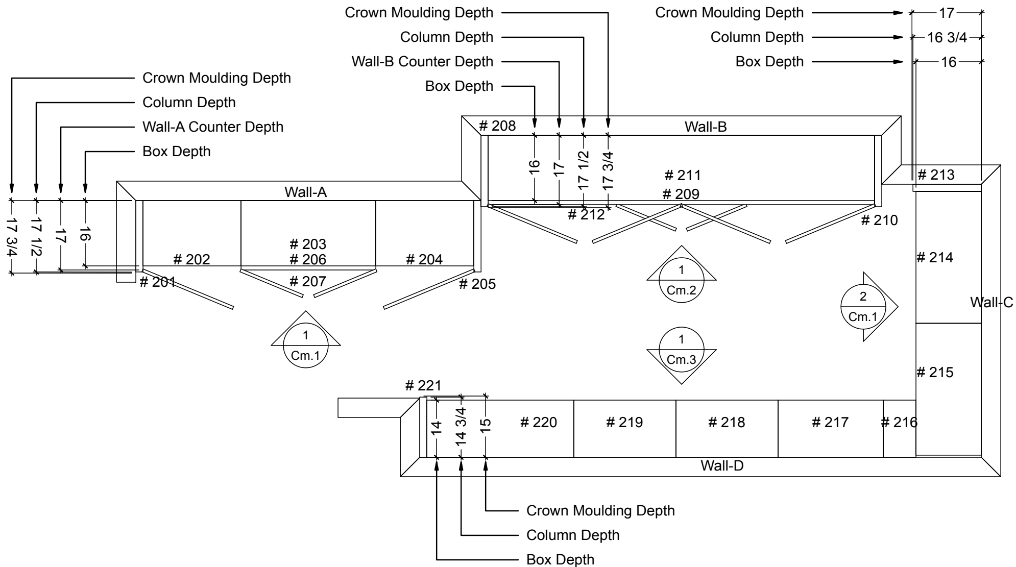
MASTER CLOSET CABINETRY FLOOR PLAN SCALE: 1/2" = 1' 0"
