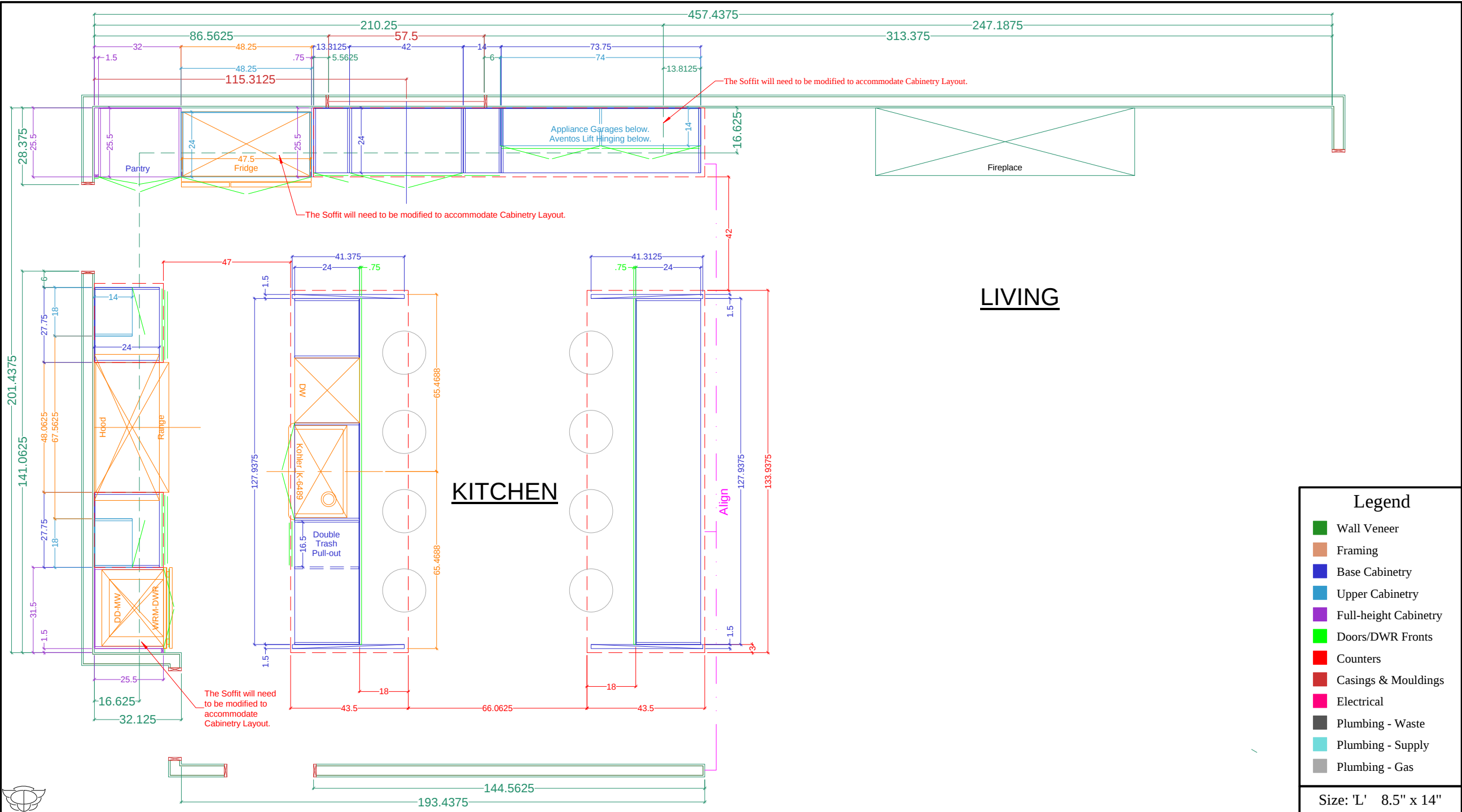
PLAN View - KITCHEN and LIVING ROOM
