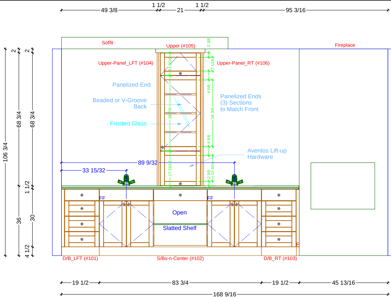
1 MASTER BATH ELEVATION SCALE: 1/2" = 1' 0"
