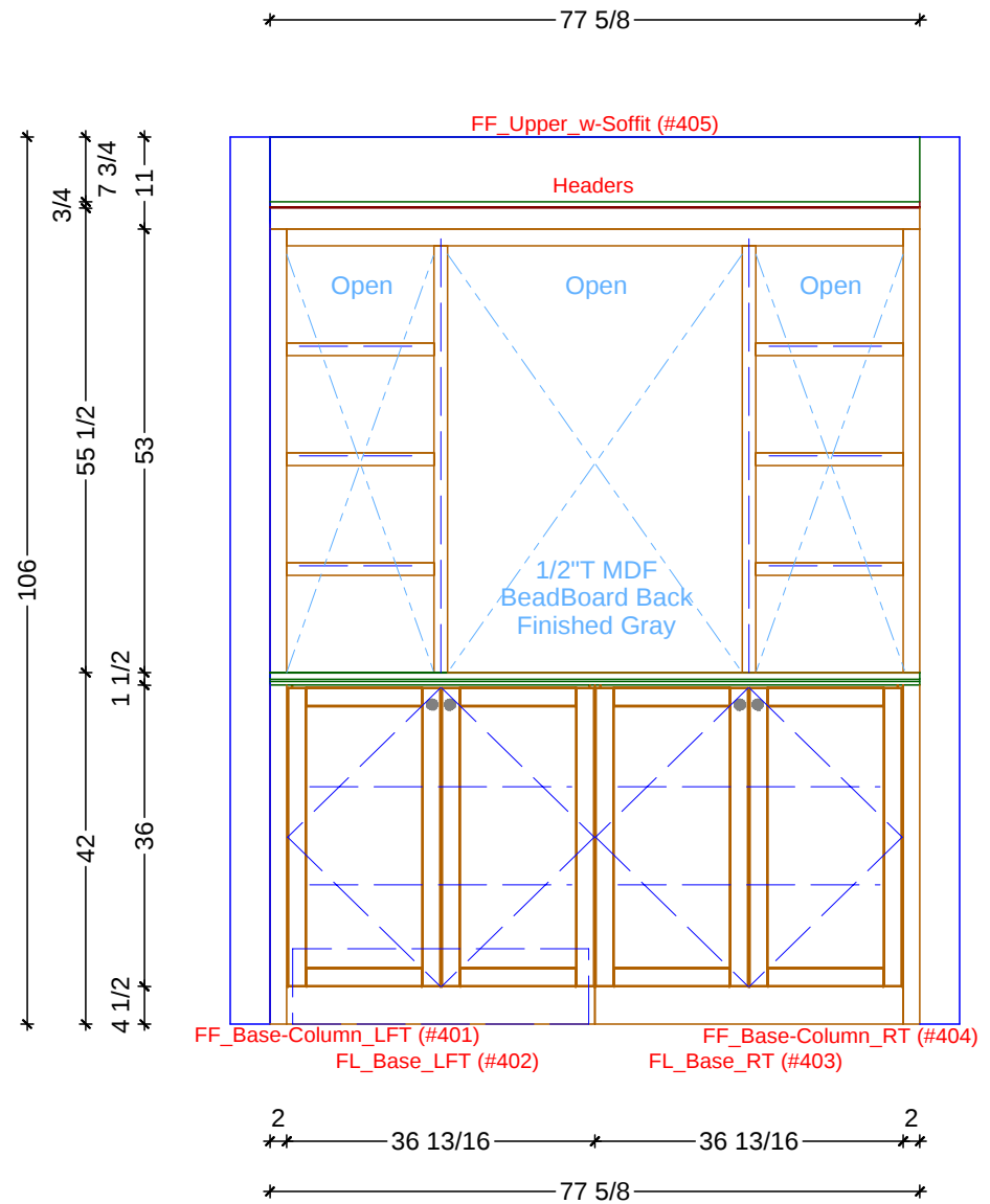
NICHE-LANDING ELEVATION SCALE: 1/2" = 1' 0"
