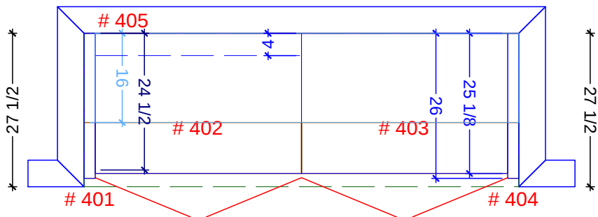
NICHE-LANDING CABINETRY FLOOR PLAN SCALE: 1/2" = 1' 0"
