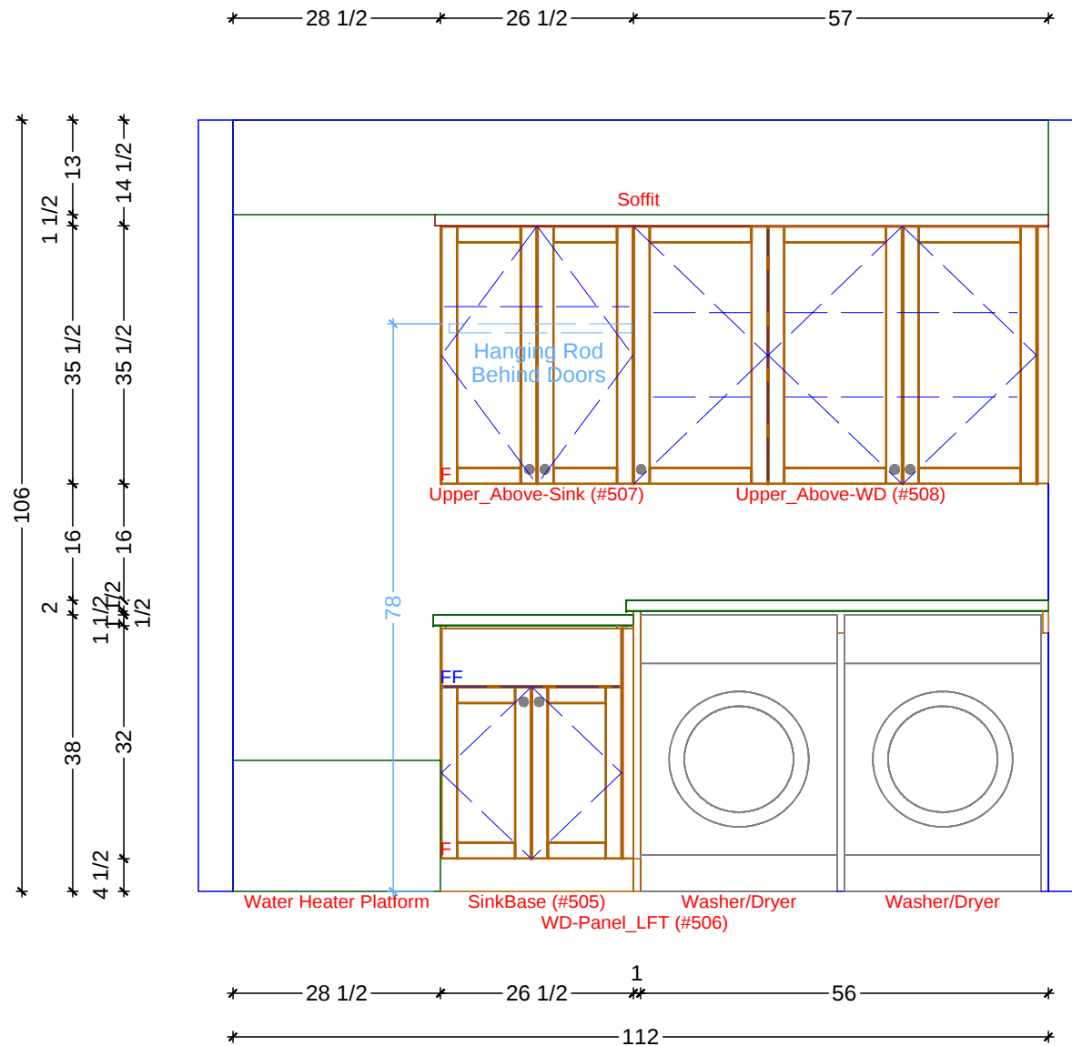
1 LAUNDRY ELEVATION - WASHER/DRYER WALL SCALE: 1/2" = 1' 0"
