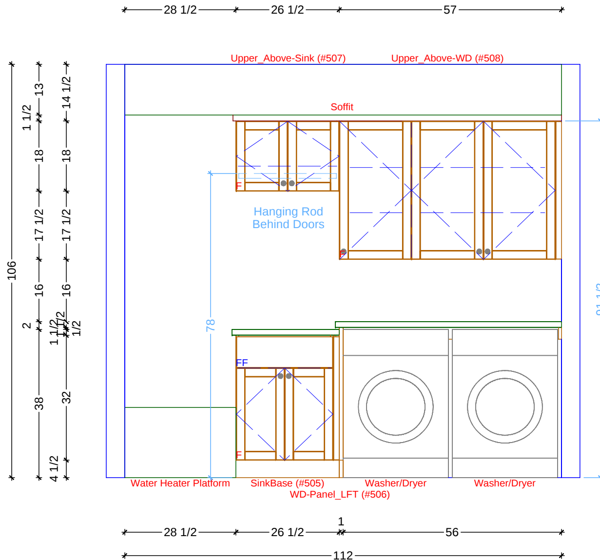
1 LAUNDRY ELEVATION - WASHER/DRYER WALL SCALE: 1/2" = 1' 0"
