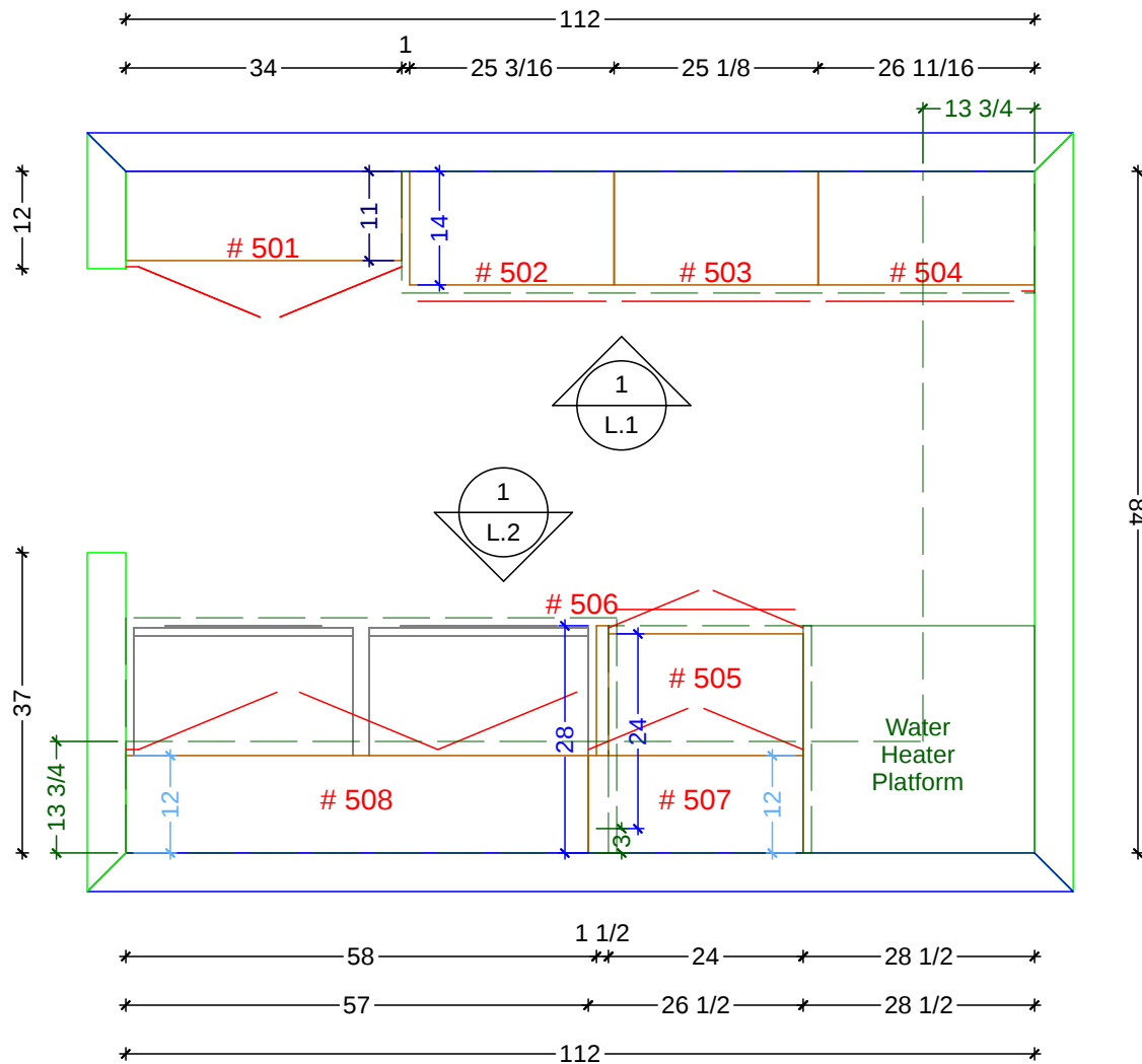
LAUNDRY CABINETRY FLOOR PLAN SCALE: 1/2" = 1' 0"
