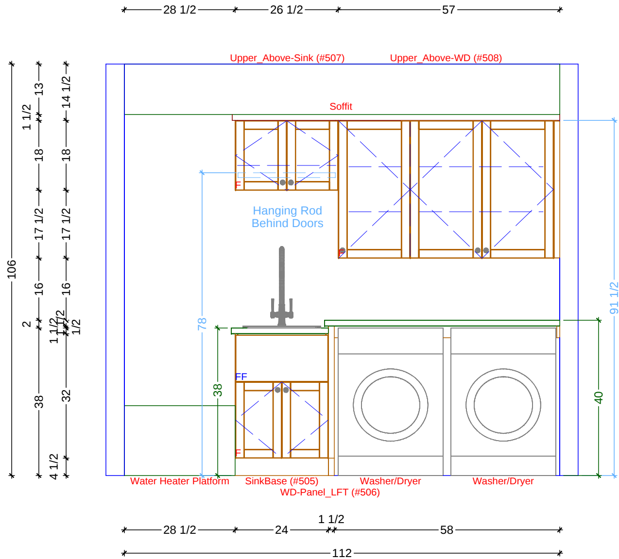
1 LAUNDRY ELEVATION - WASHER/DRYER WALL SCALE: 1/2" = 1' 0"
