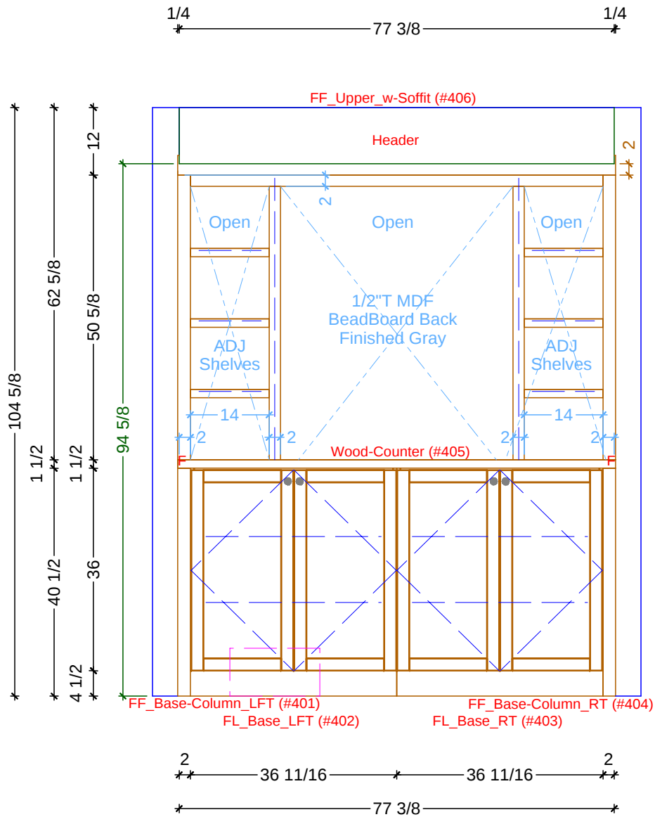
1 NICHE-LANDING ELEVATION SCALE: 1/2" = 1' 0"
