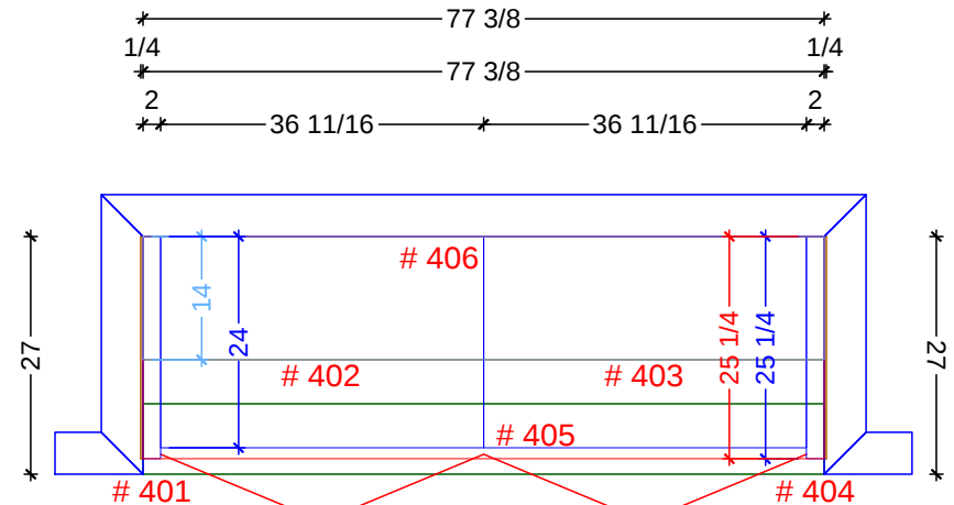
1 N-L.0 NICHE-LANDING CABINETRY FLOOR PLAN SCALE: 1/2" = 1' 0"
