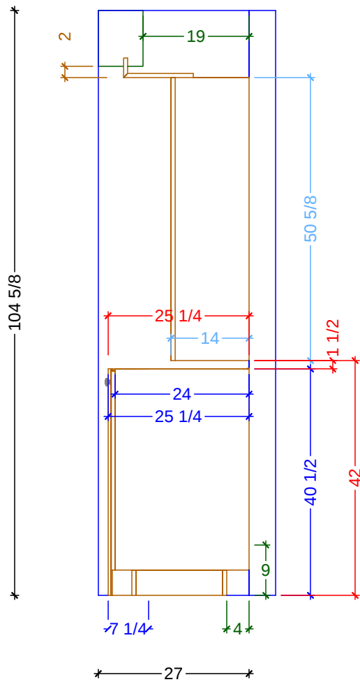
NICHE-LANDING X-SECTION SCALE: 1/2" = 1' 0"
